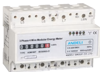
ADM100T
