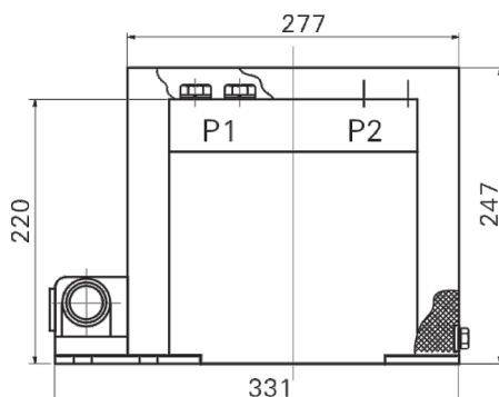
LZZBJ9-12(AS12/175b/2S)
