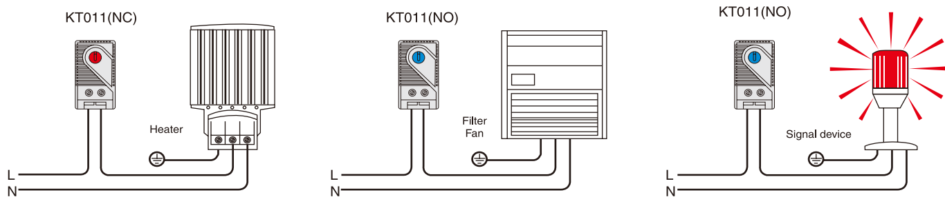
Wiring examples
