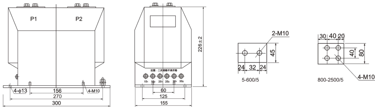
LZZBJ9-10C
