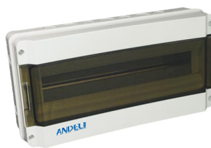
HK-18WAYS (370 x 195 x 105)
